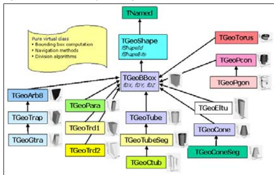
Figure 19-1 Primitive Shapes - the general inheritance scheme
