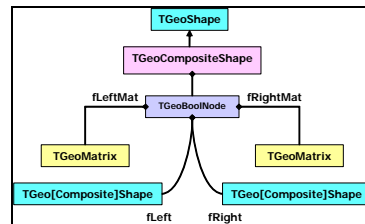
Figure 19-22 The composite shapes structure
