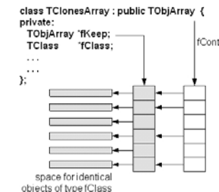
Figure 17-4 The internal data structure of a TClonesArray
