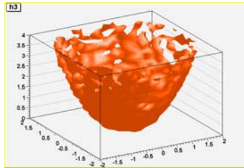
Figure 3-18 Iso surfaces
