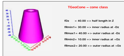
Figure 19-14 TGeoCone Class
