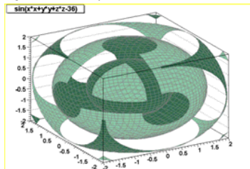
Figure 3-19 3D implicit function
