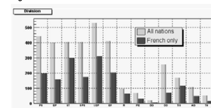
Figure 3-9 Vertical bar charts
