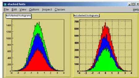
Figure 3-15 Stacked histograms
