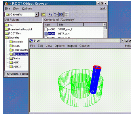
Figure 19-28 Extruding volumes
