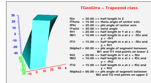
Figure 19-7 TGeoGtra class
