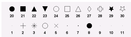
Figure 9-9 Markers
