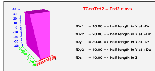
Figure 19-5 TGeoTrd2 class
