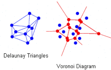
Figure 4-12 Delaunay triangles and Voronoi diagram
