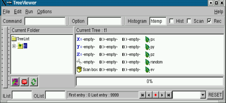
Figure 12-2 The TreeViewer
