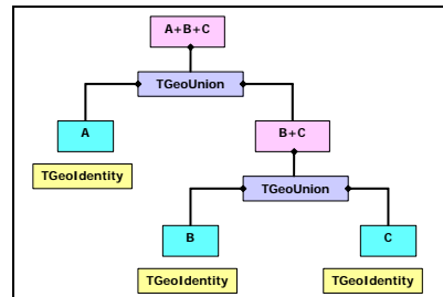
Figure 19-23 Representation of A+B+C
