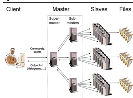
Figure 25-1 The Multi-tier structure of a PROOF cluster
