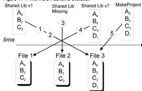
Figure 11-7 The ROOT schema evolution
