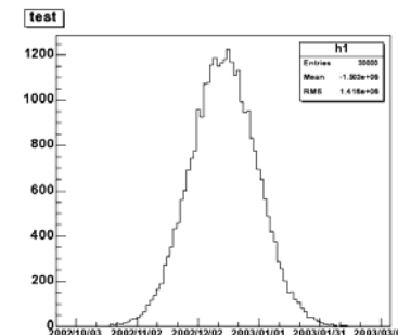
Figure 9-22 A histogram with time axis X
