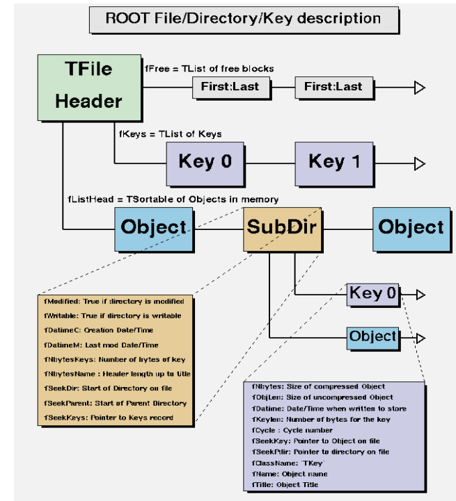
Figure 11-2 ROOT File/Directory/Key description
