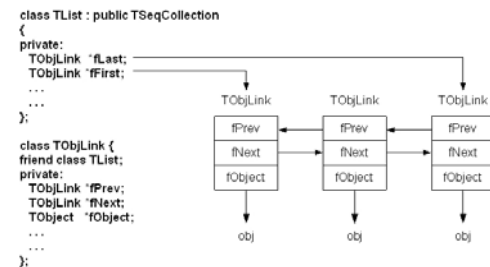
Figure 17-2 The internal data structure of a TList
