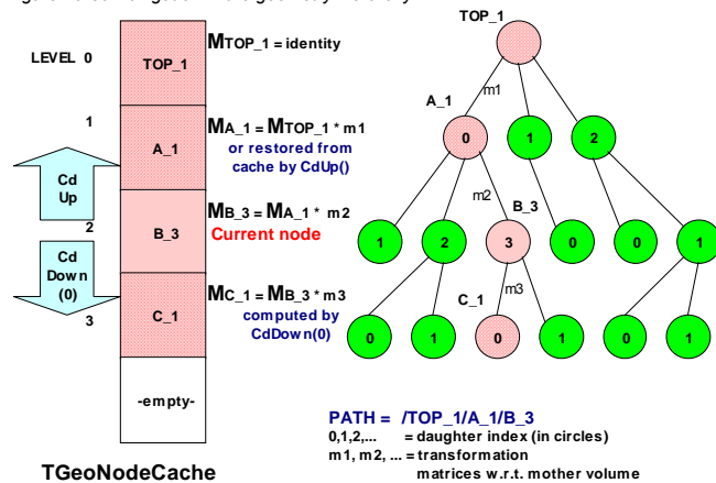
Figure 19-35 Navigation in the geometry hierarchy
