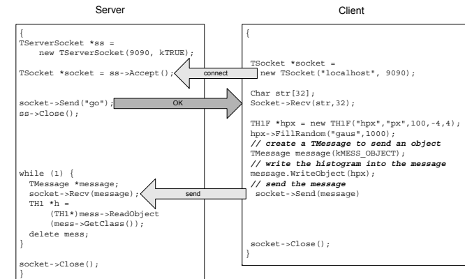
Figure 23-1 Server - Client setting-up and closing the connection
