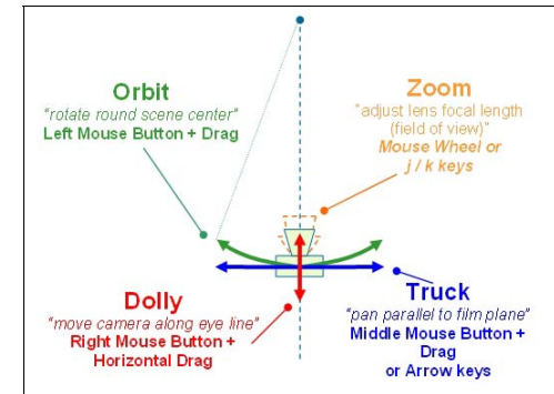
Figure 9-33 GL Viewer camera interactions
