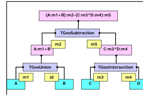
Figure 19-24 Internal representation for composite shapes
