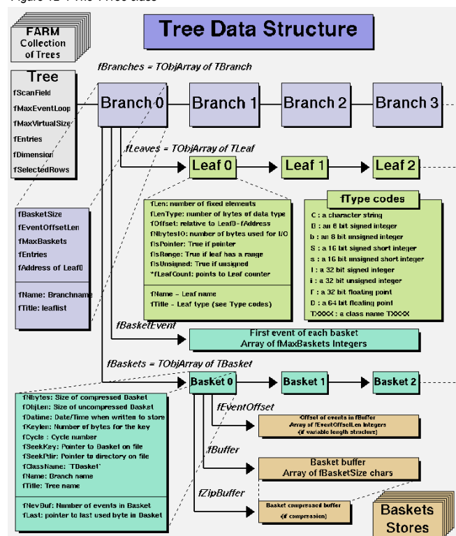
Figure 12-4 The TTree class
