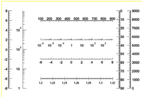
Figure 9-23 The first axis example
