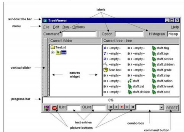
Figure 26-1 Widgets created by ROOT GUI classes
