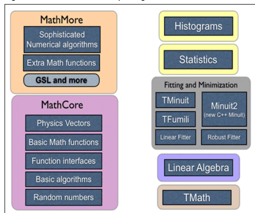
Figure 13-1 Math libraries and packages
