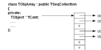
Figure 17-3 The internal data structure of a TObjArray
