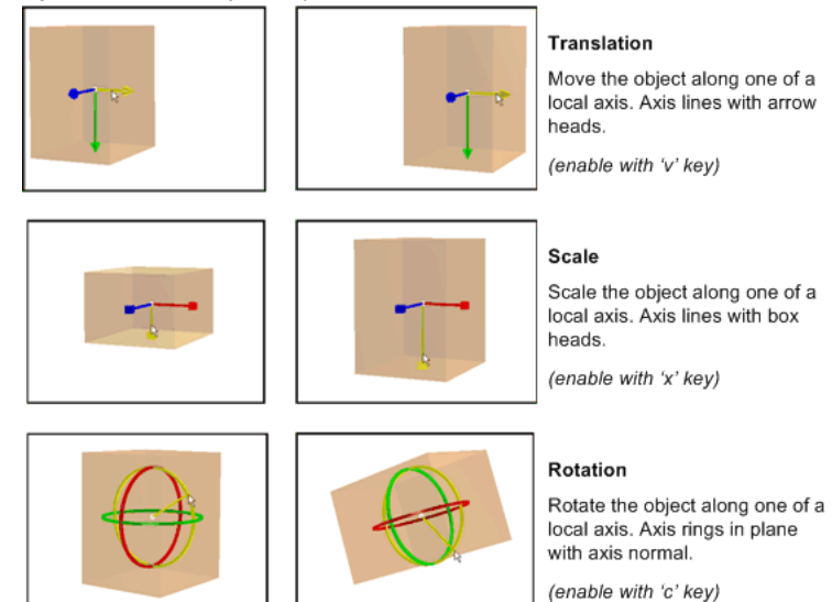
Figure 9-36 GL Viewer object manipulators
