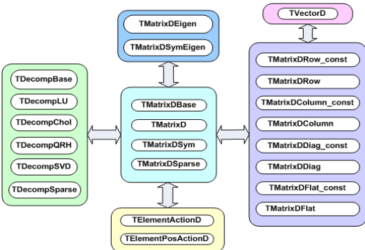
Figure 14-1 Overview of matrix classes
