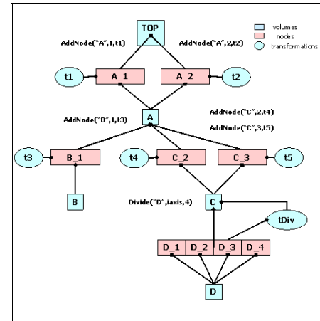
Figure 19-26 A geometry hierarchy in memory
