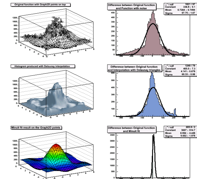
Figure 4-14 Output of macro graph2dfit.C
