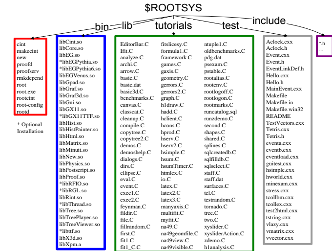
Figure 1-1 ROOT framework directories
