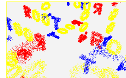
Figure 19-31 Random points
