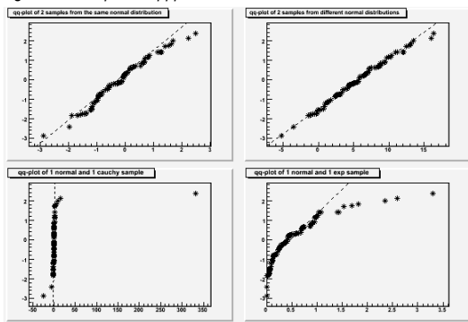
Figure 4-9 Examples of qq-plots of 2 datasets
