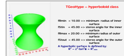
Figure 19-13 TGeoHype Class
