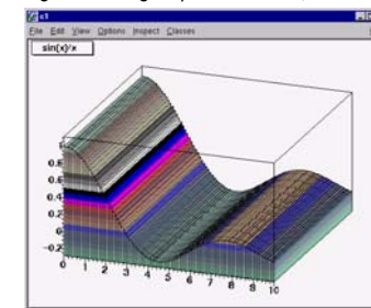
Figure 2-4 "Lego2" plot of \sin(x)/x
