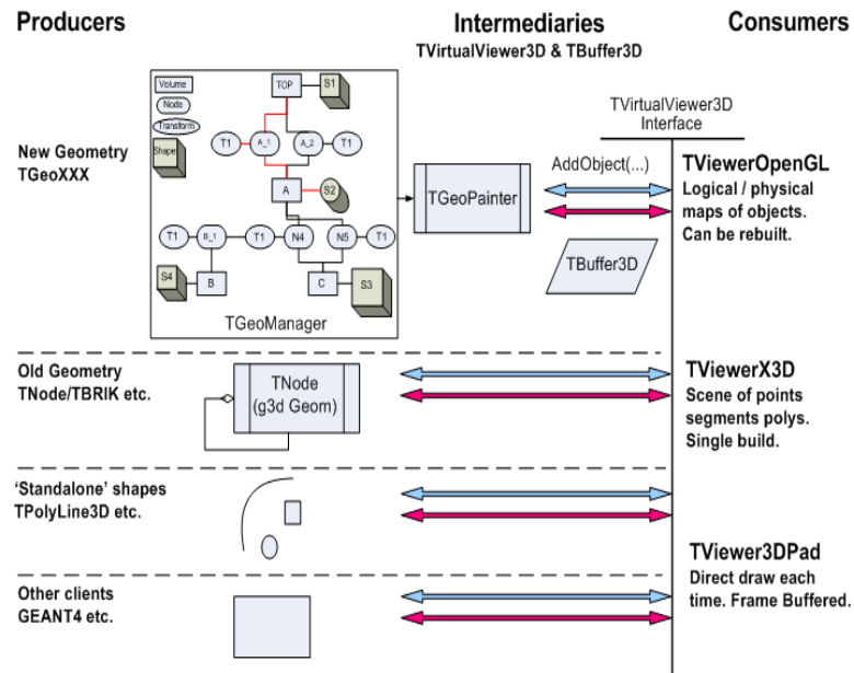
Figure 9-37 Overview of 3D viewer architecture
