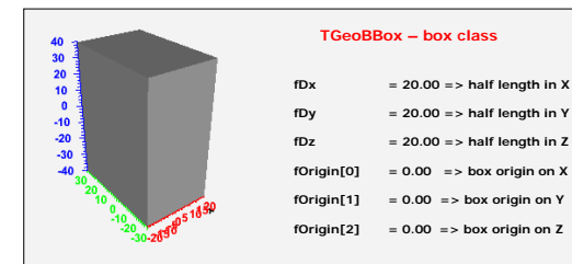
Figure 19-2 TGeoBBox class
