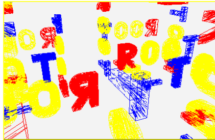
Figure 19-32 Random rays
