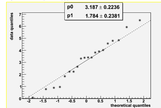
Figure 4-10 Examples of qq-plots of 1 dataset
