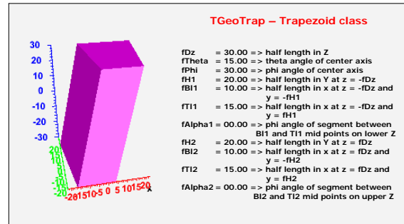
Figure 19-6 TGeoTrap Class
