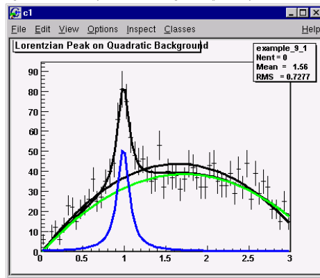
Figure 5-3 The output of the FittingDemo() example
