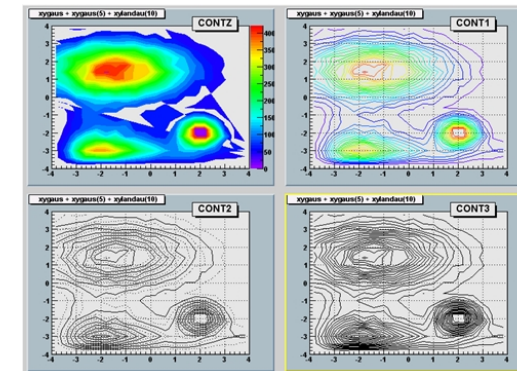
Figure 3-5 Different contour options
