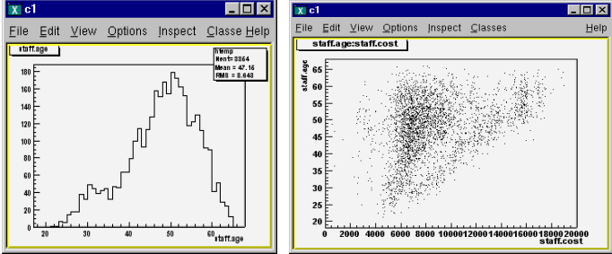
Figure 12-3 A couple of graphs
