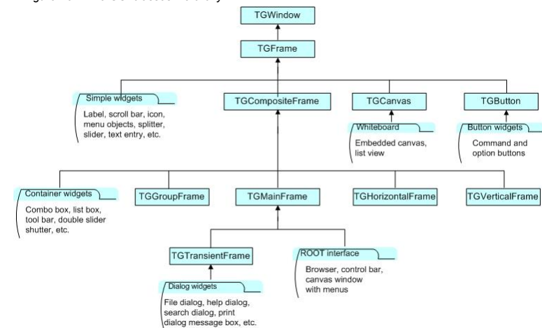
Figure 26-2 The GUI classes hierarchy
