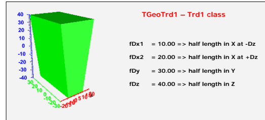
Figure 19-4 TGeoTrd1 class
