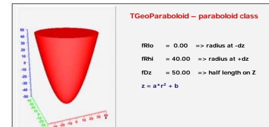
Figure 19-18 TGeoParaboloid Class
