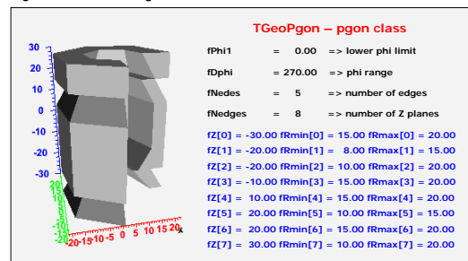
Figure 19-20 TGeoPgon Class
