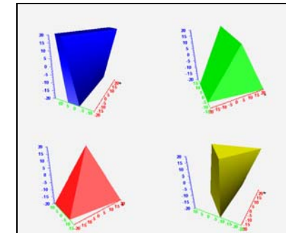
Figure 19-8 TGeoArb8 class
