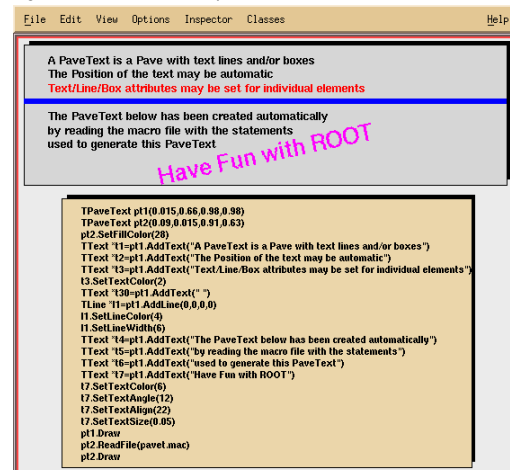
Figure 9-17 PaveText examples
