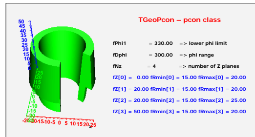
Figure 19-19 TGeoPcon Class
