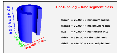
Figure 19-10 TGeoTubeSeg Class
