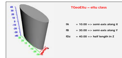
Figure 19-12 TGeoEltu Class
