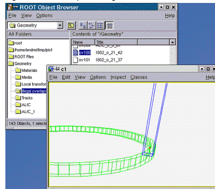
Figure 19-29 Overlap checking
