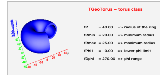
Figure 19-17 TGeoTorus Class
