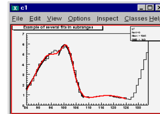
Figure 5-2 Fitting a histogram with several Gaussian functions
