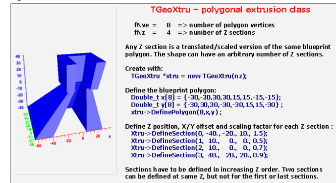
Figure 19-21 TGeoXtru Class
