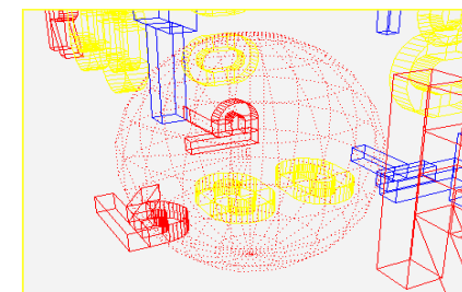
Figure 19-31 Random points
