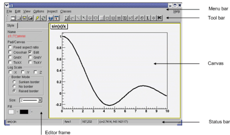
Figure 2-1 A canvas with drawing
