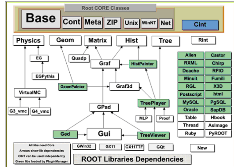
Figure 1-2 ROOT libraries dependencies
