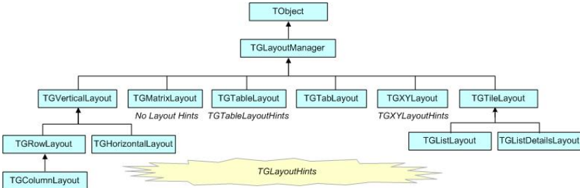
Figure 26-3 The layout classes hierarchy
