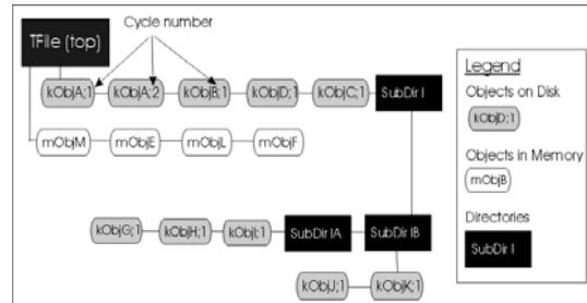
Figure 11-3 The structure of TFile
