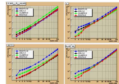
Figure 14-2 Speed comparison between the different matrix packages
