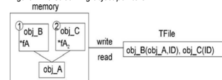
Figure 11-6 Streaming object pointers
