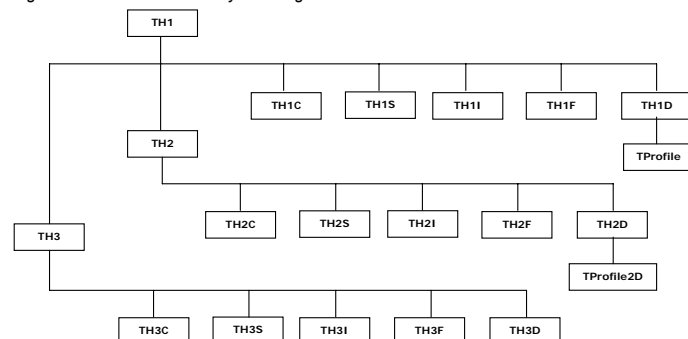
Figure 3-1 The class hierarchy of histogram classes
