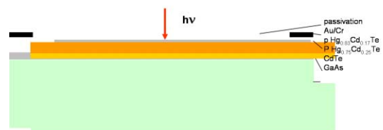
Figure 2 – Schematic cross section of an uncooled IR Hg 1-x Cd x Te photodetector.
