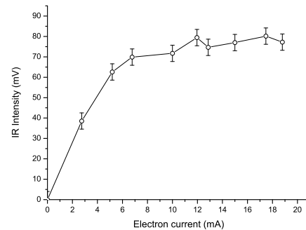
Figure 6: IR signal vs. the electron current.
