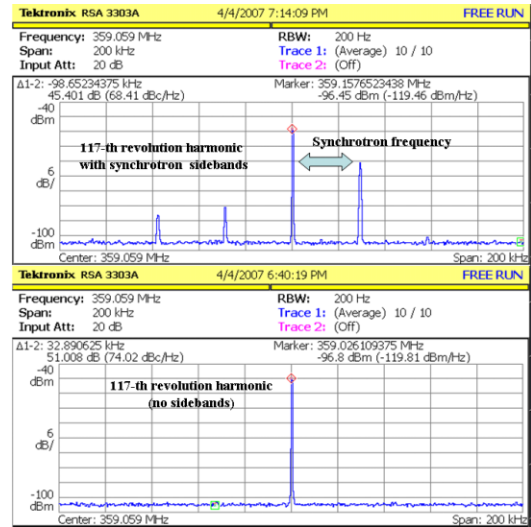
Figure 5: Upper panel: 106 bunches with 734 mA e^- beam current and longitudinal feedback off . Lower panel: 106 bunches with 1227 mA e^- beam current with longitudinal feedback on .
