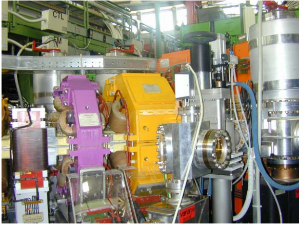
Figure 7: Photo of the exit port recently installed at one of the bending magnet of the DAΦNE positron ring.
