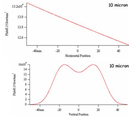
Figure 9: Vertical and horizontal intensity distributions of the IR source simulated at 20 cm from the window.
