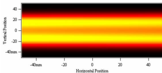
Figure 8: Simulation of the intensity distribution of the DAΦNE bending magnet IR emission at the wavelength of 10 \mu\text{m} .
