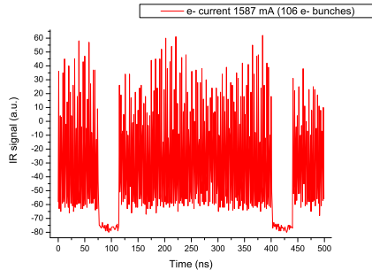
Figure 3: The DAΦNE electron bunches structure as detected by a fast IR uncooled device.
