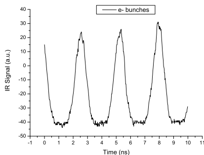
Figure 4: IR signal of three adjacent electron bunches.
