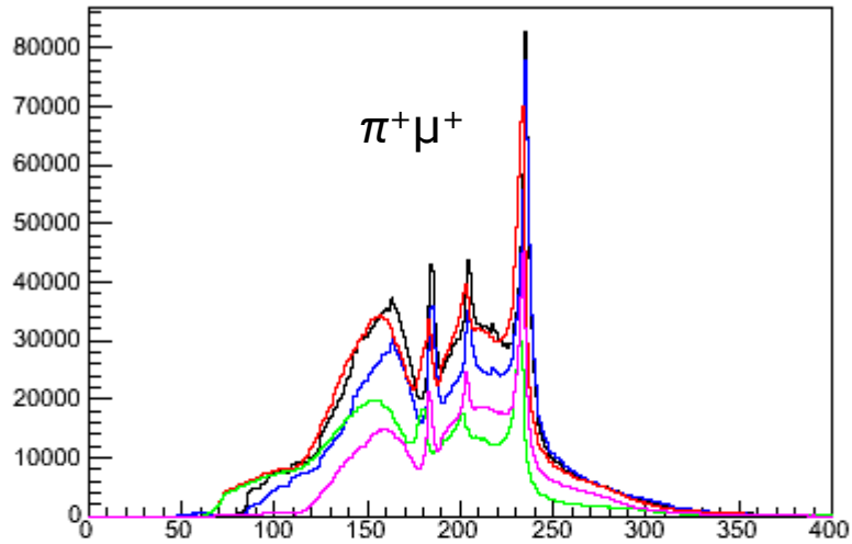
DEDXmmomm {DEDXmextm == 1}
