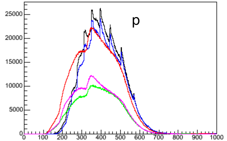
DEDXpmomp {DEDXpextp == 1}
