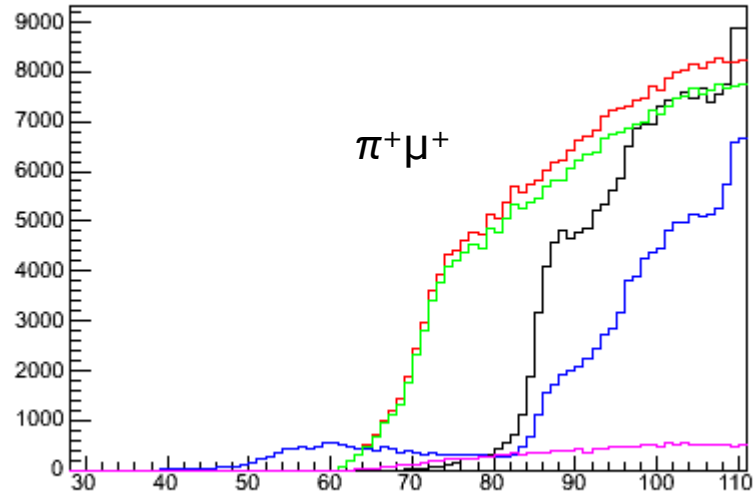
DEDXmmomm {DEDXmextm == 1}
