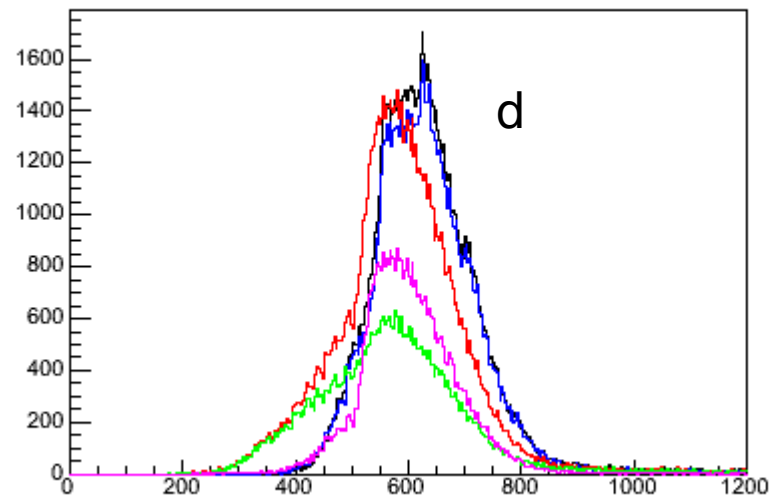
DEDXdmomd {DEDXdextd == 1}
