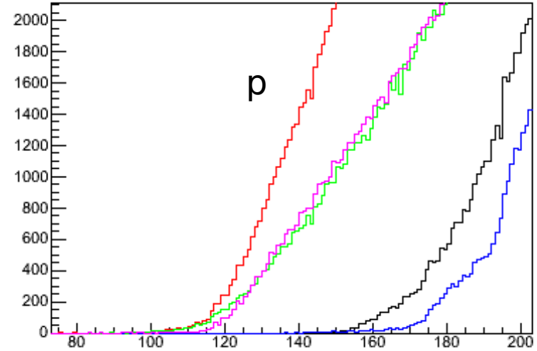
DEDXpmomp {DEDXpextp == 1}
