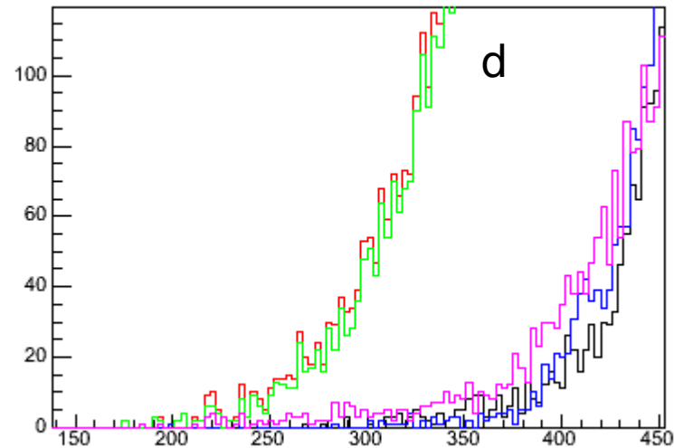
DEDXdmomd {DEDXdextd == 1}
