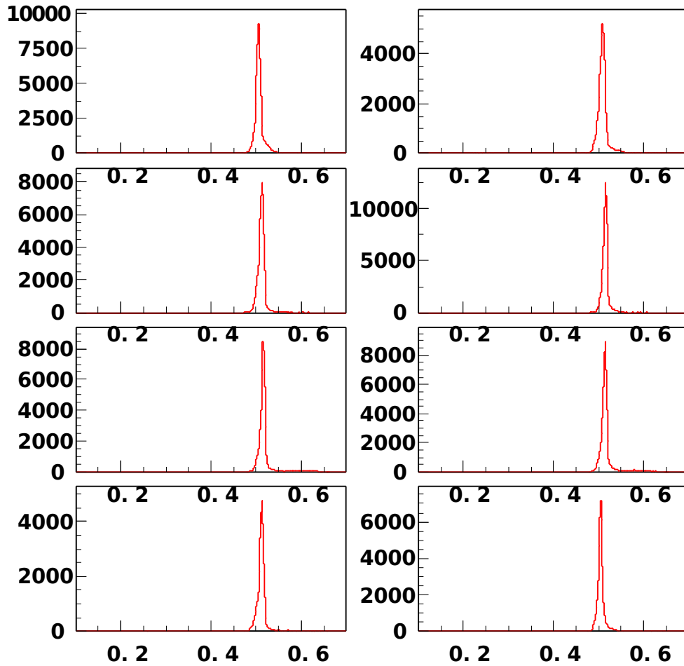
Electrons
