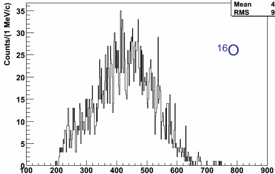
Momentum of protons 6
