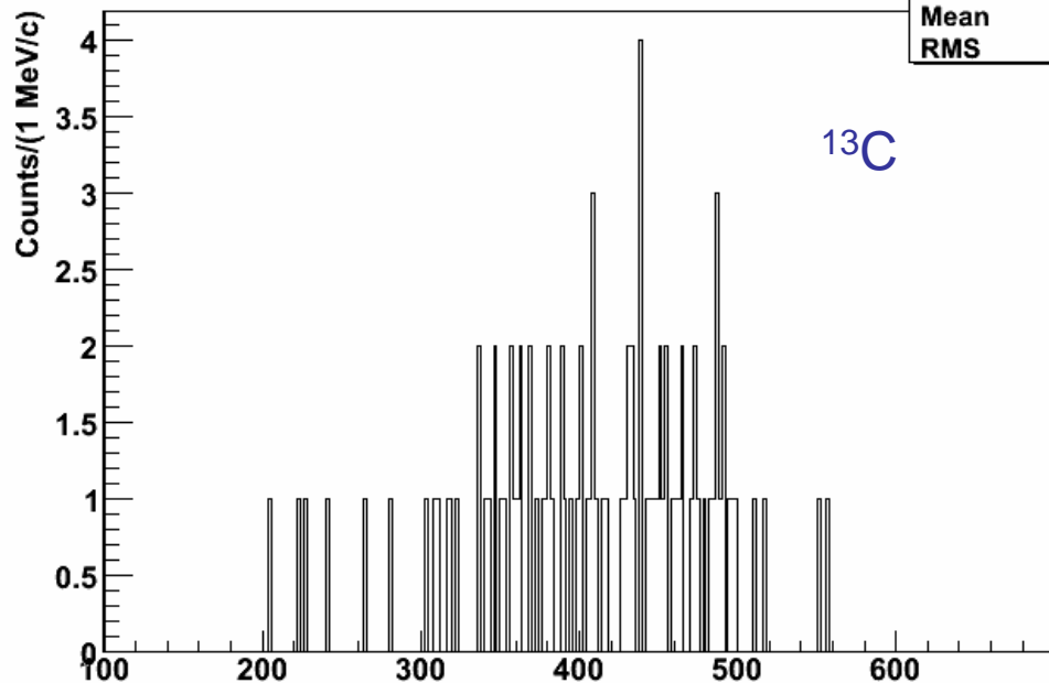
Momentum of protons in coincidence with a fast pion 4
