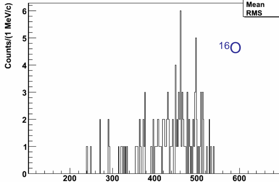
Momentum of protons in coincidence with a fast pion 6
