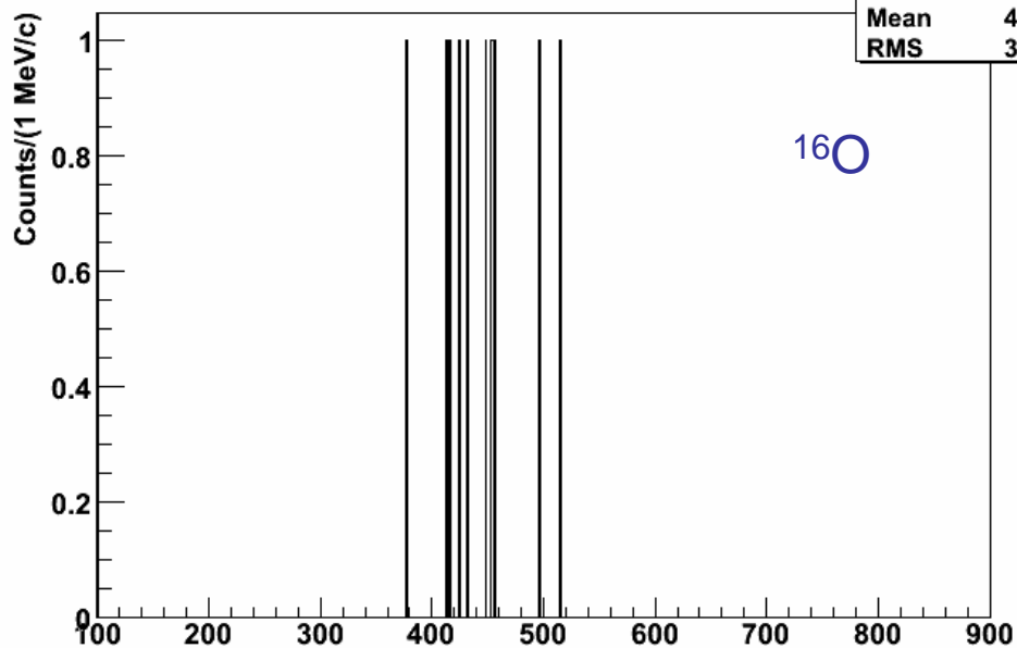
Momentum of protons in coincidence with a fast pion 6
